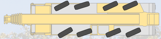
Variable steering concept Concept de direction variable
